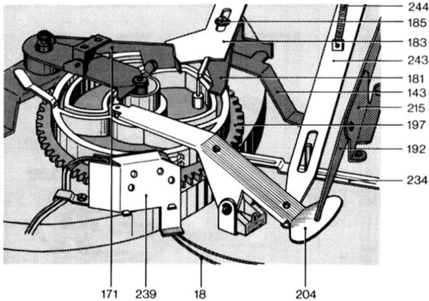
Fig. 10 Tonearm guide mechanism
