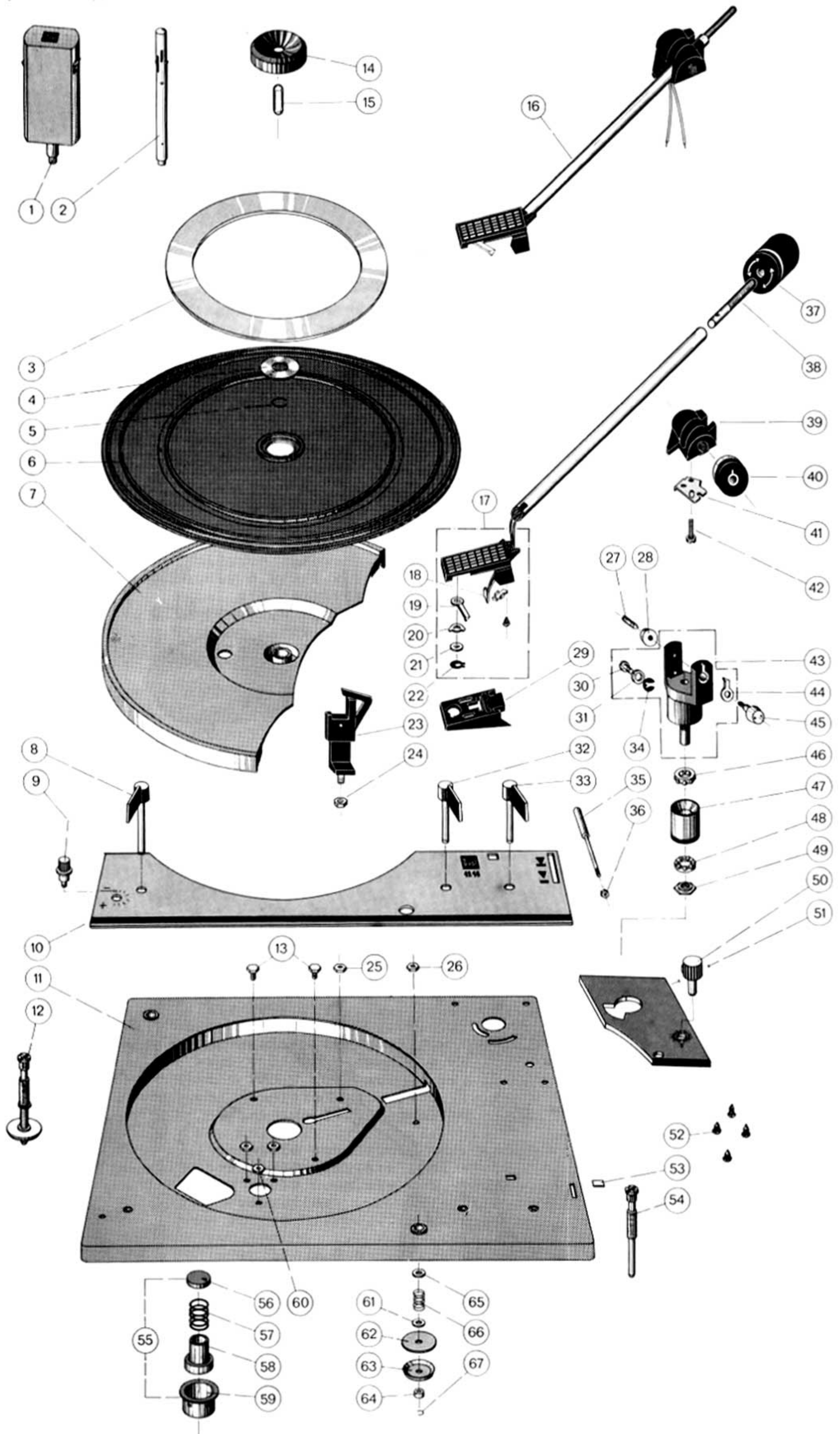
Fig. 24 Exploded view, parts above chassis
